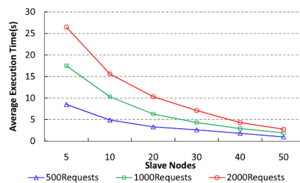
FIGURE 19. Performance evaluation of the HQR system.
