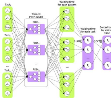
FIGURE 2. Parallelization recommendation process of the HQR system.
