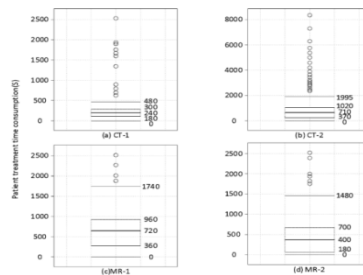
FIGURE 14. Noisy data removal results for the PTTP algorithm.
